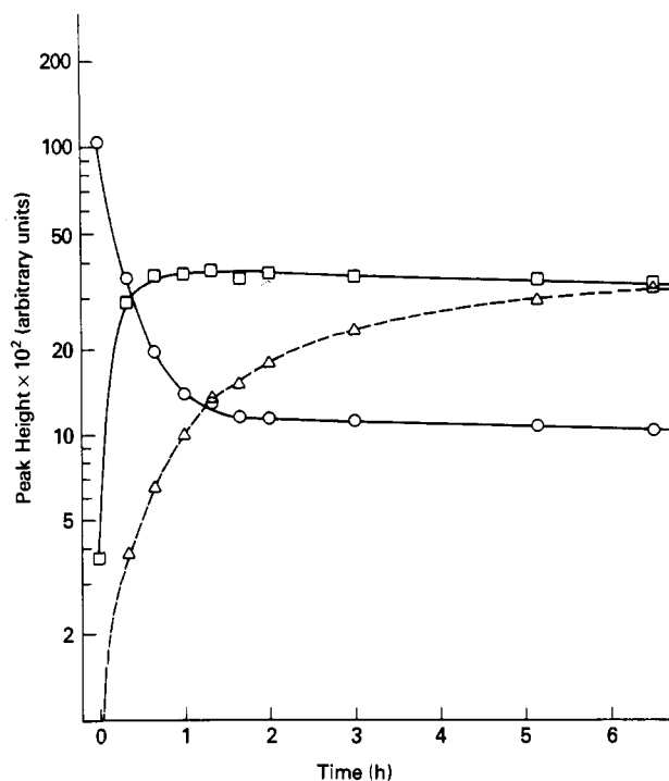
Figure 2. The furanose-pyranose isomerization of model compound 6 in pH 1 HCl buffer at 25^{\circ}\text{C} . Mixture components were separated by reverse-phase HPLC and monitored at 215 nm (see Experimental Section). Key: (O) ribofuranoside 6, (□) ribopyranoside 7, (Δ) ribopyranoside 16a.
